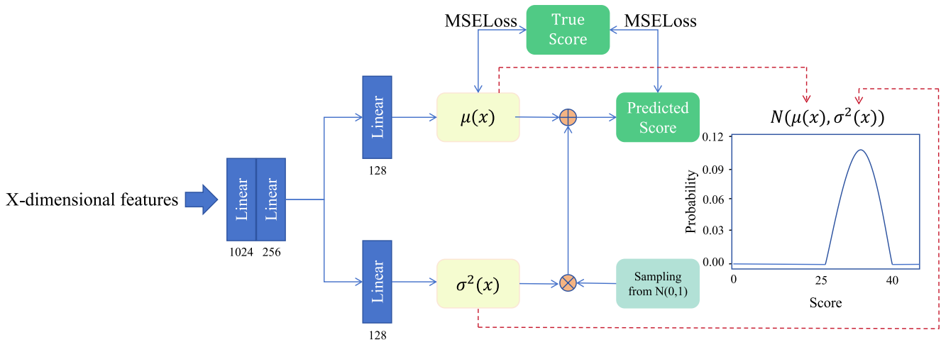
FIGURE 7 | Architecture diagram for score prediction.
